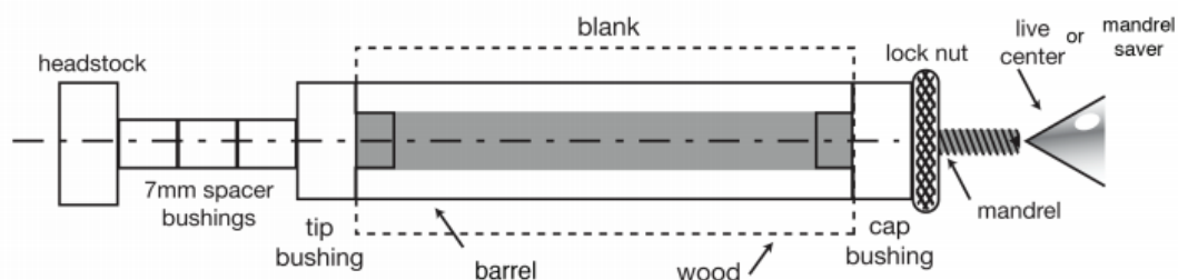
DIAGRAM B • Turning the blank
