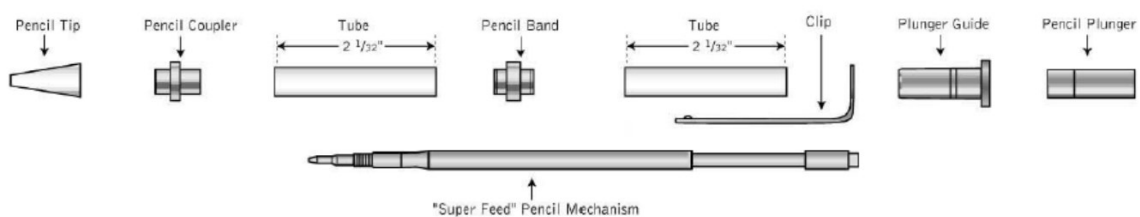
Diagram B: PENCIL PARTS
