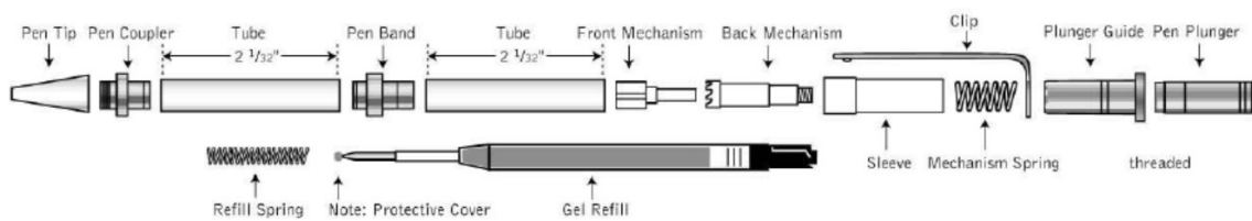
Diagram A: PEN PARTS
