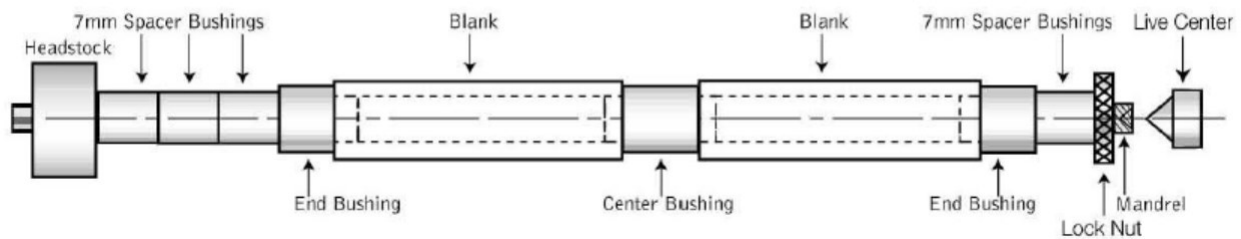
Diagram C: TURNING THE BLANKS
